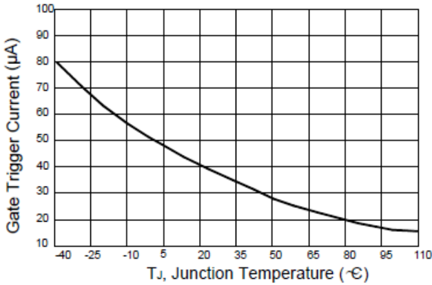
Figure 1. Typical Gate Trigger Current Versus Junction Temperature
