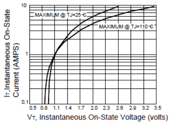
Figure 6. Typical On-State Characteristics
